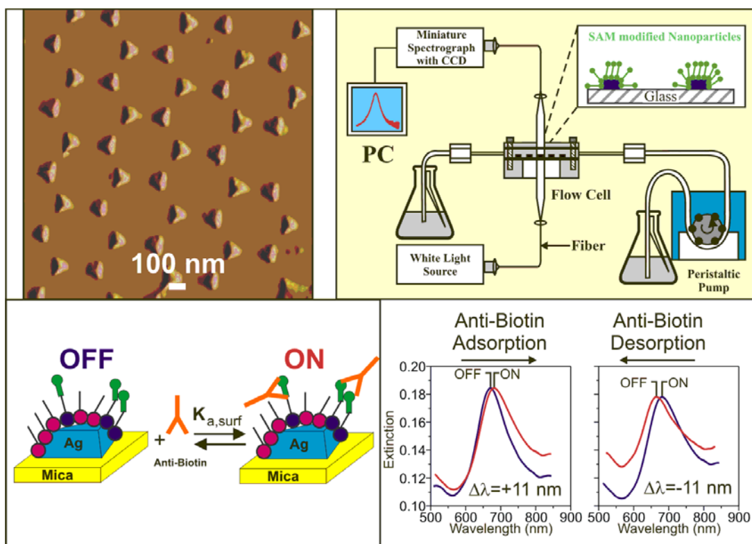
Localized Surface Plasmon Resonance Immunoassay: Ag nanoparticle array (upper left), instrumental setup (upper right), schematic representation of the surface chemistry (lower left), reversible LSPR immunoassay (lower right).
